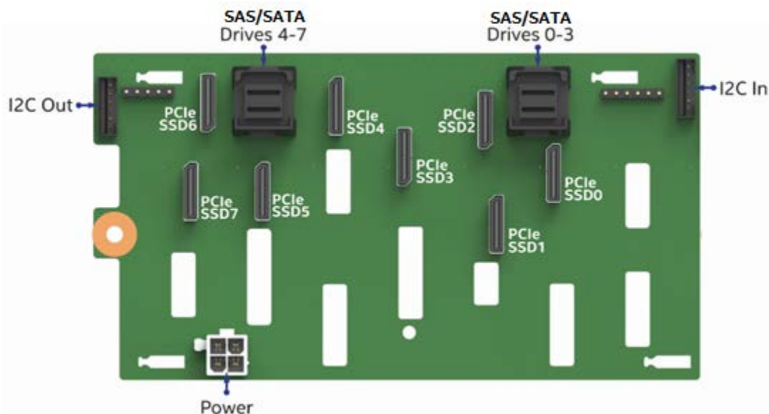
Figure 52. 8 x 2.5" SAS/SATA/NVMe* hot swap backplane, back side
