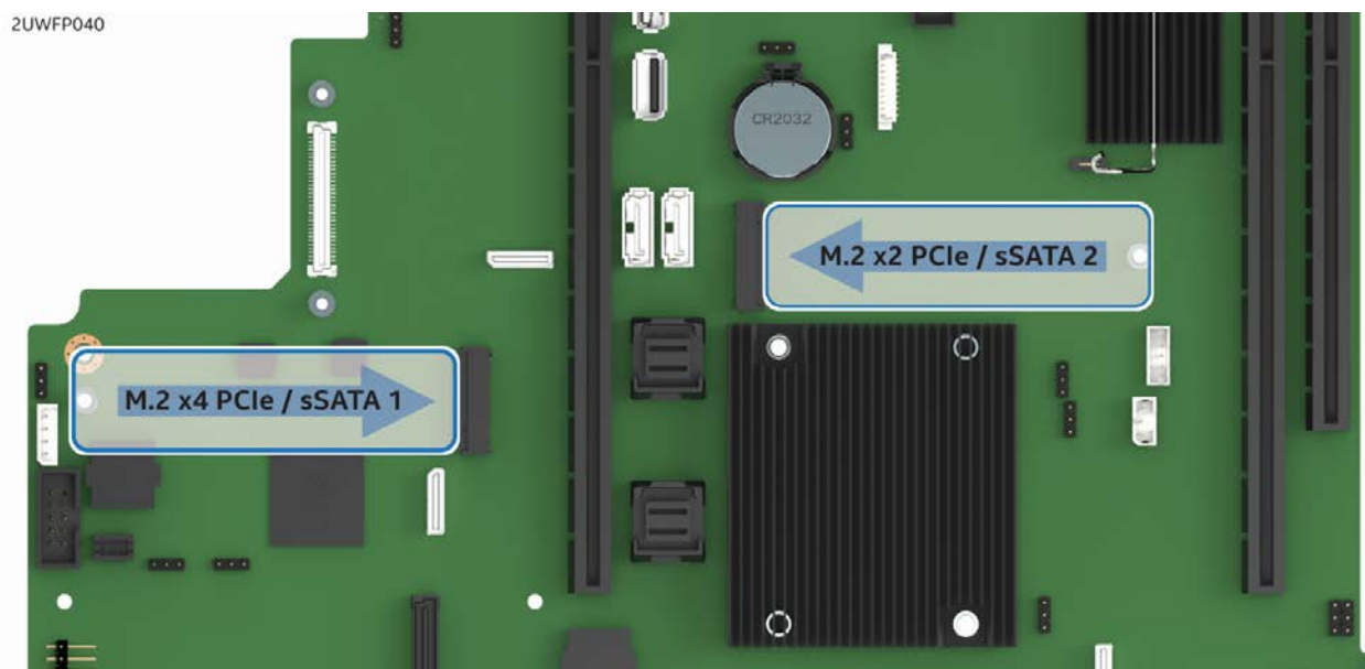
Figure 65. M.2 module connector locations
