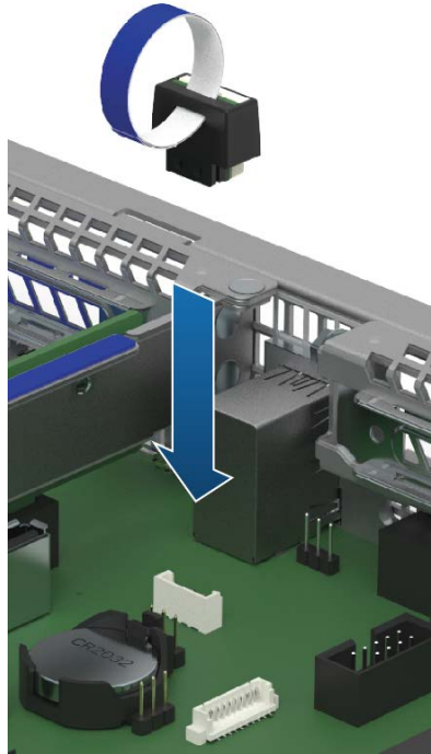
Figure 64. Intel® ESRT2 SATA RAID-5 upgrade key
