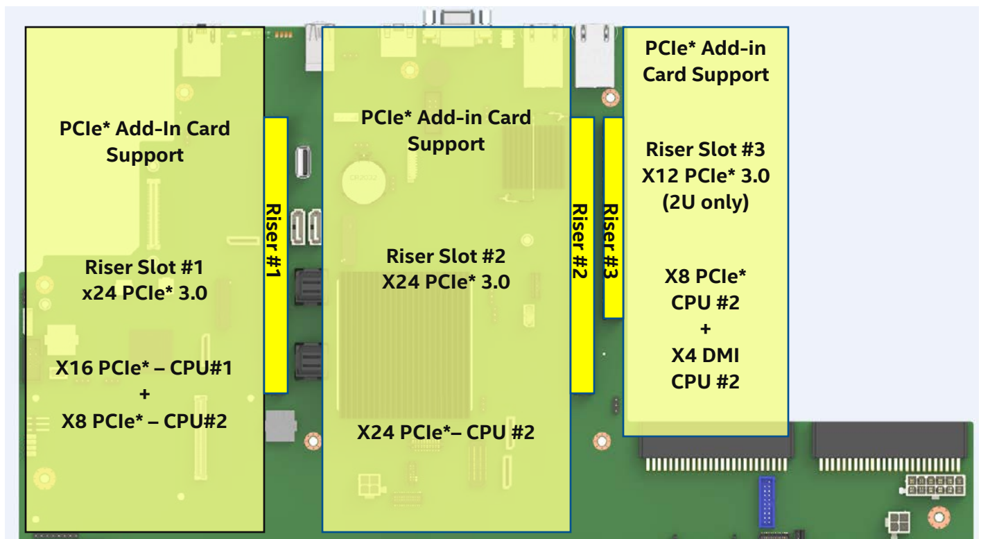
Figure 85. PCIe* add-in card support
