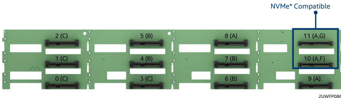
Figure 57. 12 x 3.5" hot swap backplane, front side
