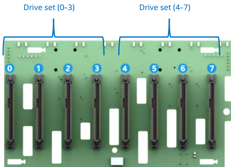
Figure 75. Drive set and connector identification
