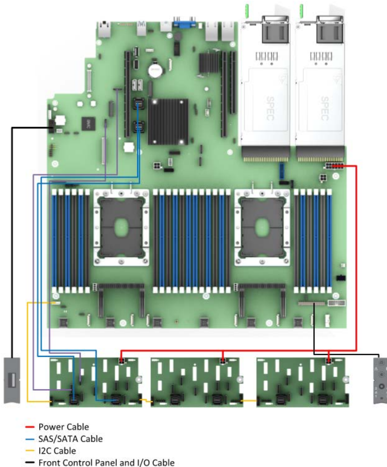
Figure 100. R2224WFxxx system cable routing diagram
