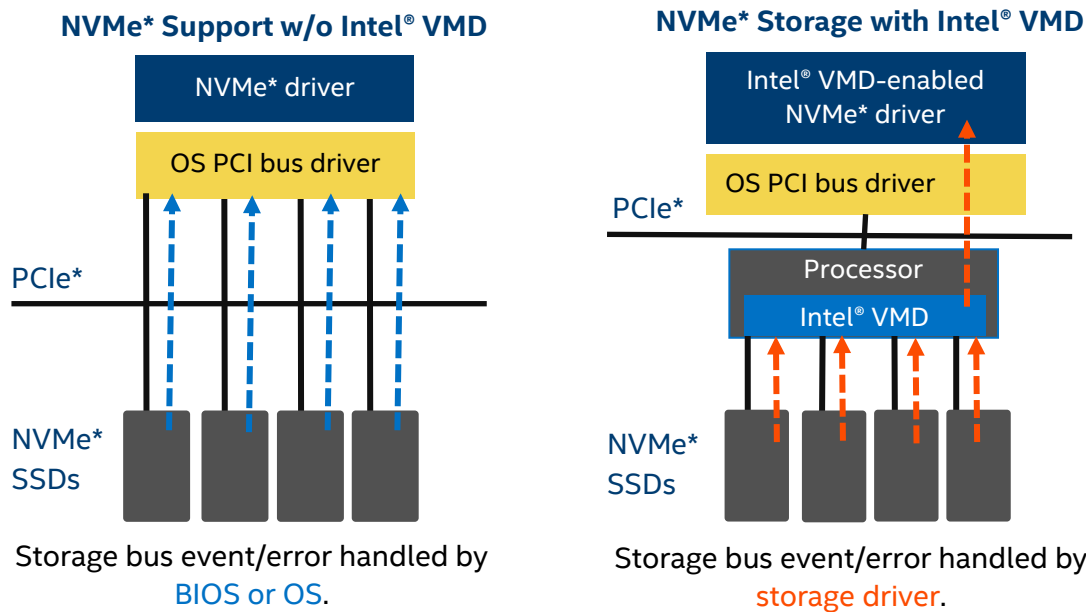
Figure 67. NVMe* storage bus event/error handling
