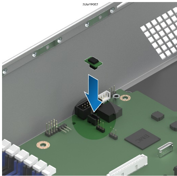
Figure 93. Intel® RMM4 Lite activation key placement
