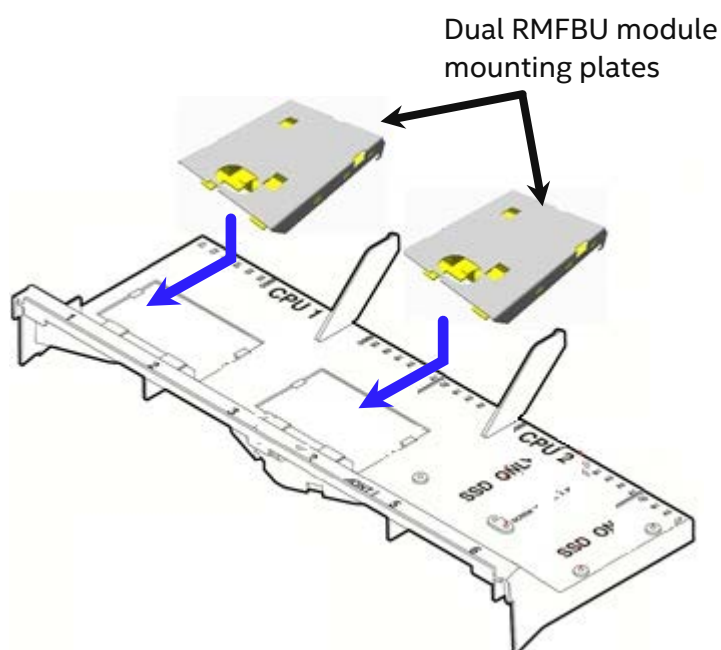
Figure 79. Dual RMFBU mounting bracket installation
