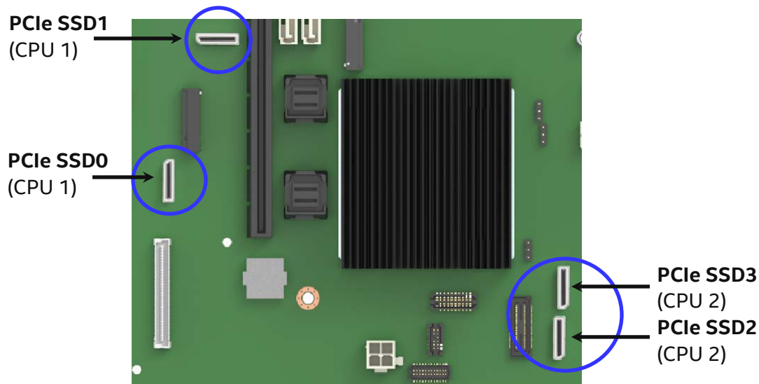
Figure 66. Onboard OCuLink connectors
