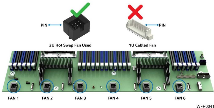
Figure 34. Server board 2U system fan connector locations
