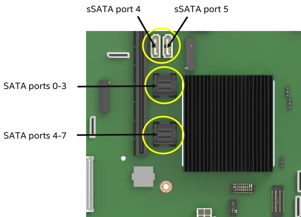
Figure 62. Onboard SATA port connector identification
