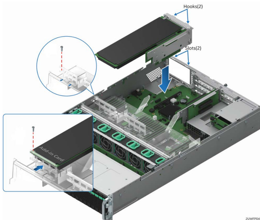
Figure 88. Full-height/full-length add-in card support
