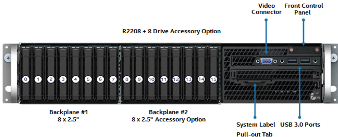
Figure 40. 2.5" front mount drive bay, 8-drive (R2208WFXXX) and 16-drive configuration
