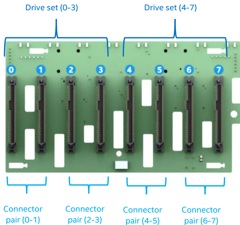
Figure 73. Drive set and connector identification
