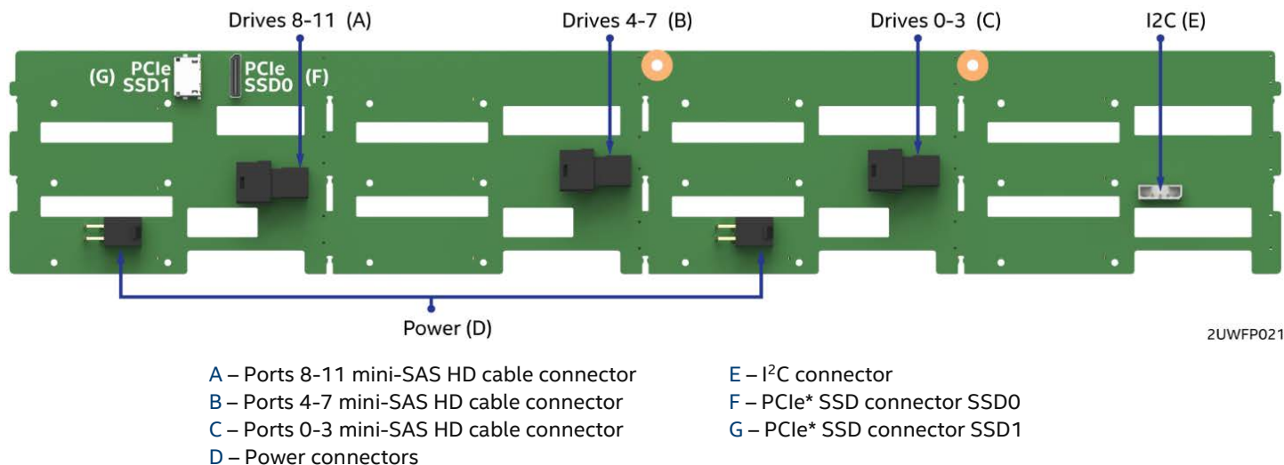
Figure 58. 12 x 3.5" HSBP connector identification
