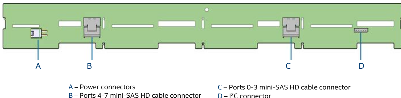
Figure 56. 8 x 3.5" HSBP connector identification
