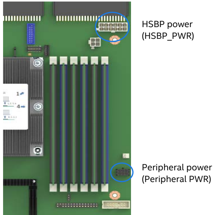
Figure 48. Server board peripheral power connectors
