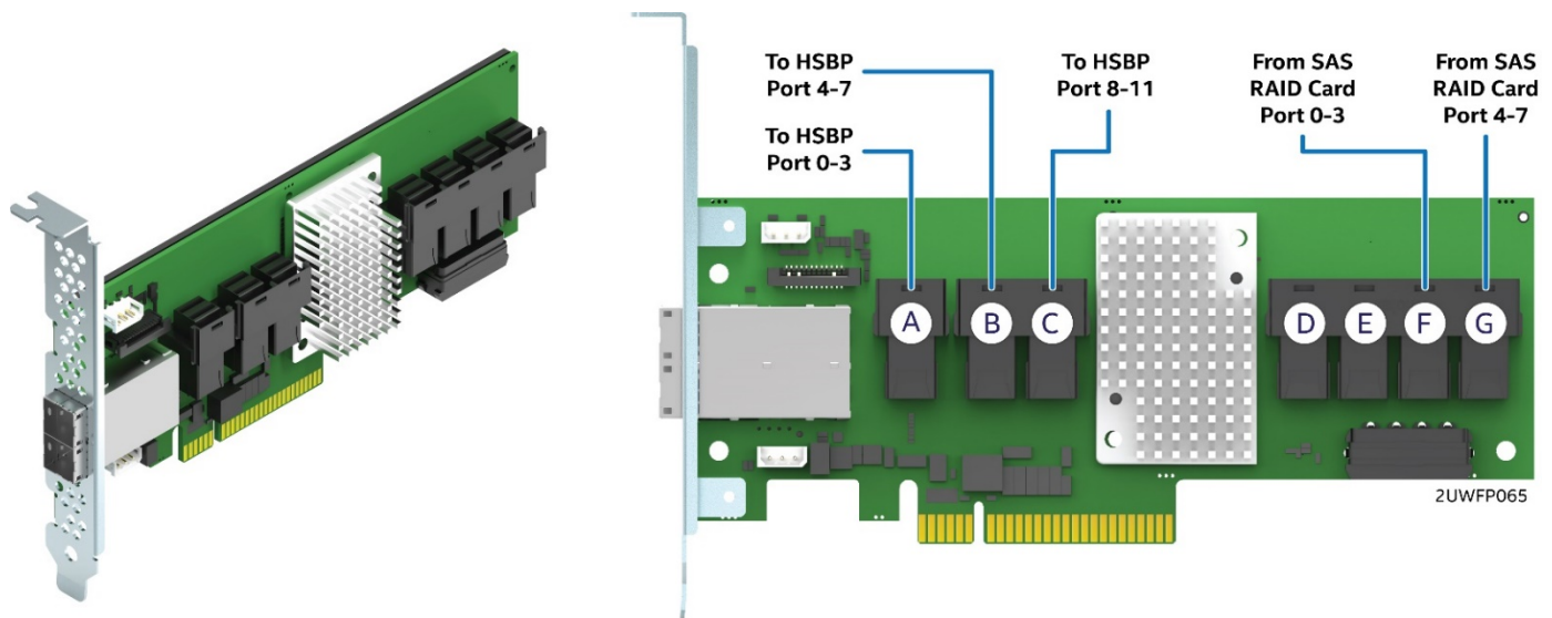
Figure 81. Intel® RAID Expander RES3FV288 connector identification
