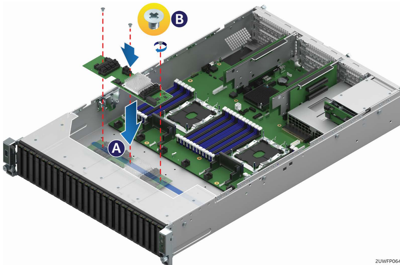
Figure 80. SAS expander card installation
