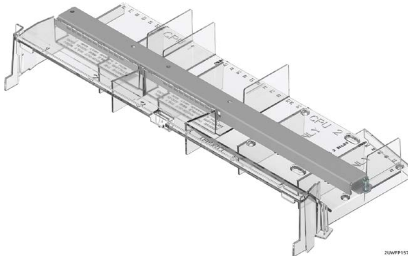
Figure 39. Shipping bracket placement
