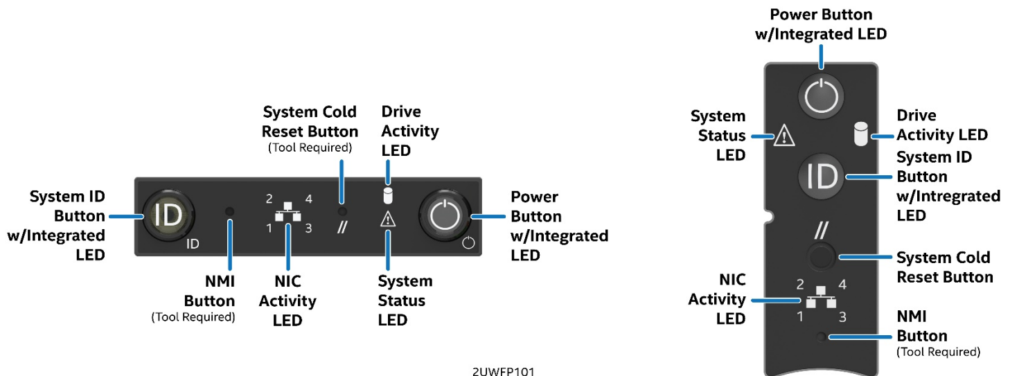
Figure 84. Front control panel features
