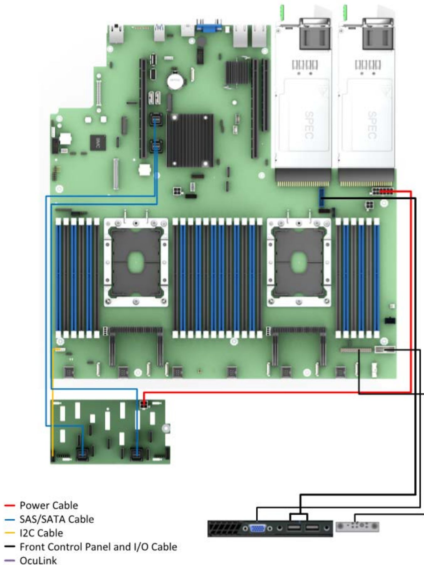
Figure 97. R2208WFxxx system cable routing diagram
