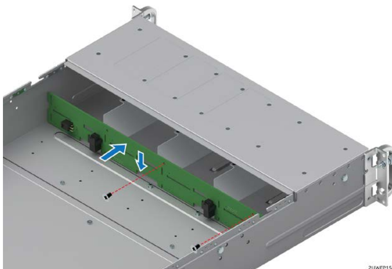
Figure 49. 3.5" backplane placement
