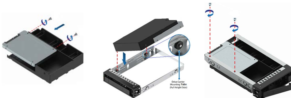
Figure 46. 2.5" SSD mounted to 3.5" drive carrier
