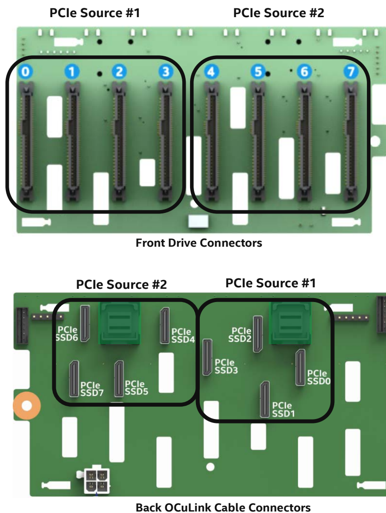
Figure 72. Backplane cabling from two PCIe* sources
