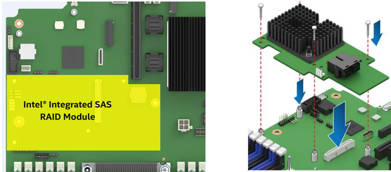
Figure 77. Intel® Integrated RAID Module
