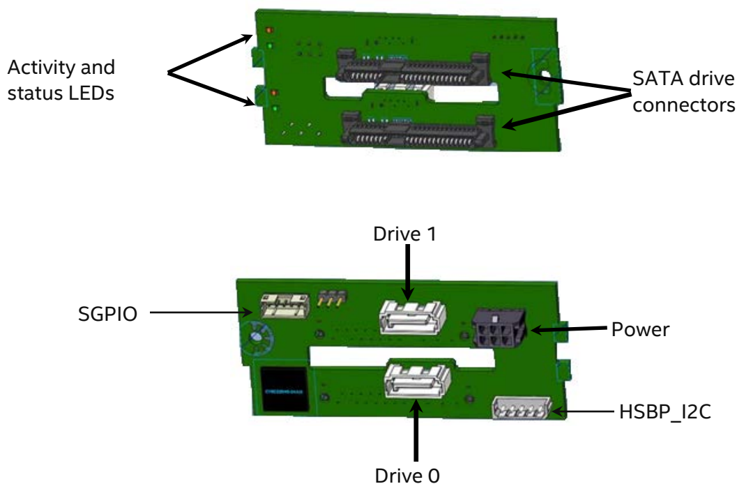
Figure 60. 2 x 2.5" hot swap backplane
