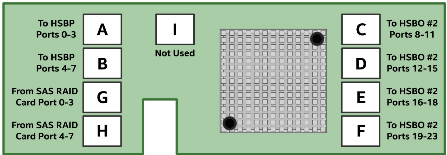
Figure 82. 12 GB internal 36-Port Intel® RAID Expander Card RES3TV360 connector identification
