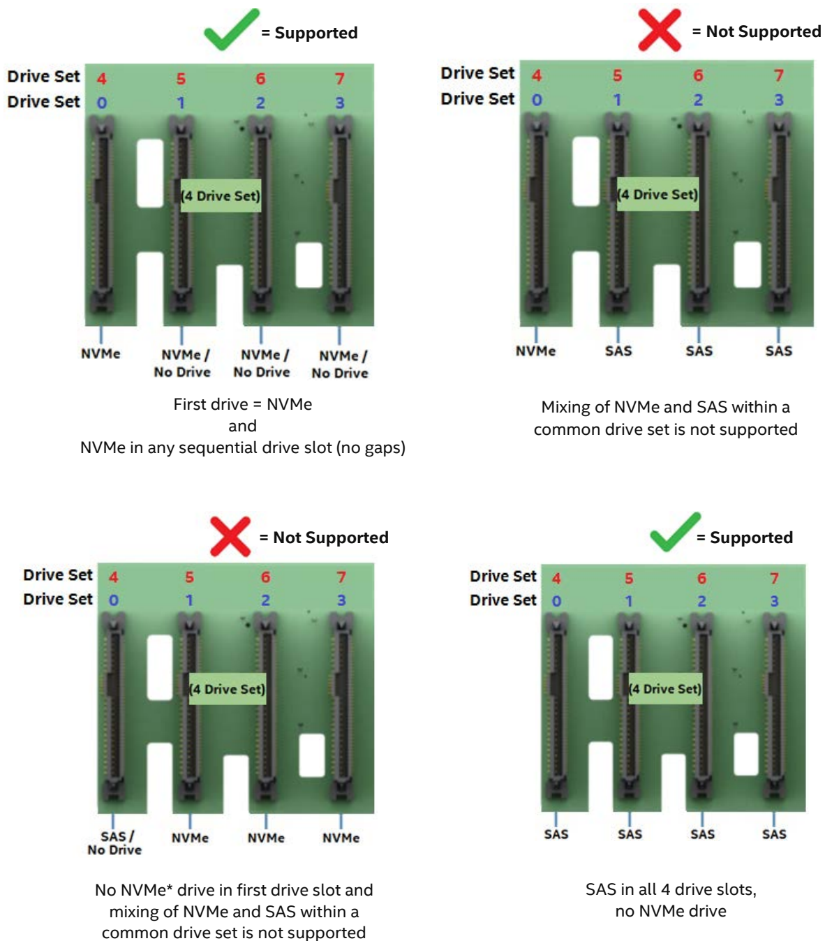
Figure 76. Supported drive population for 4- or 8-port PCIe*switch
