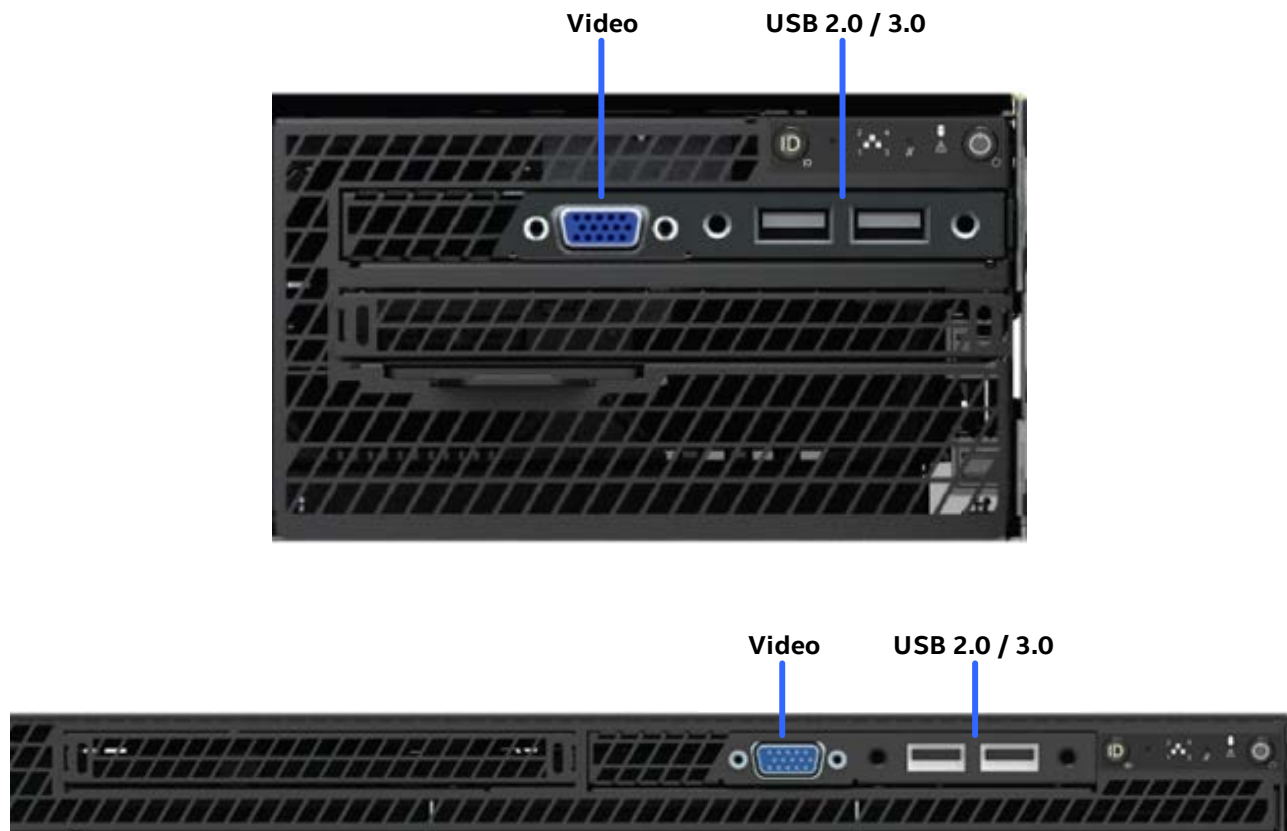
Figure 83. Front I/O panel features
