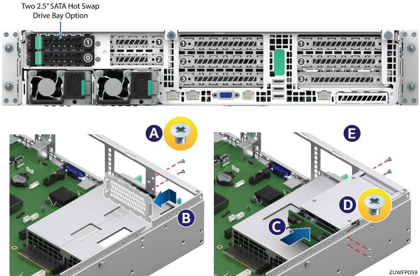
Figure 59. 2 x 2.5" rear mount backplane kit placement
