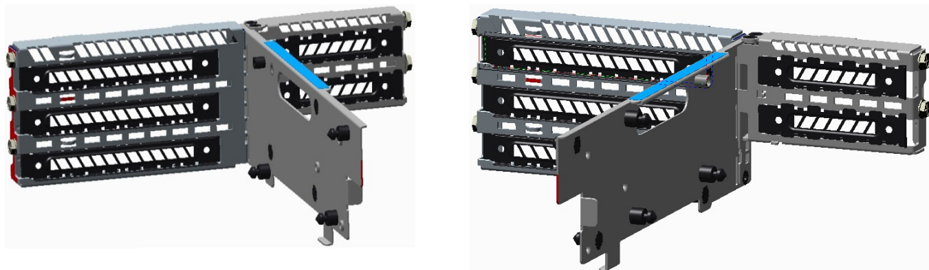
Figure 87. Left and right views of riser card #2 and #3 bracket
