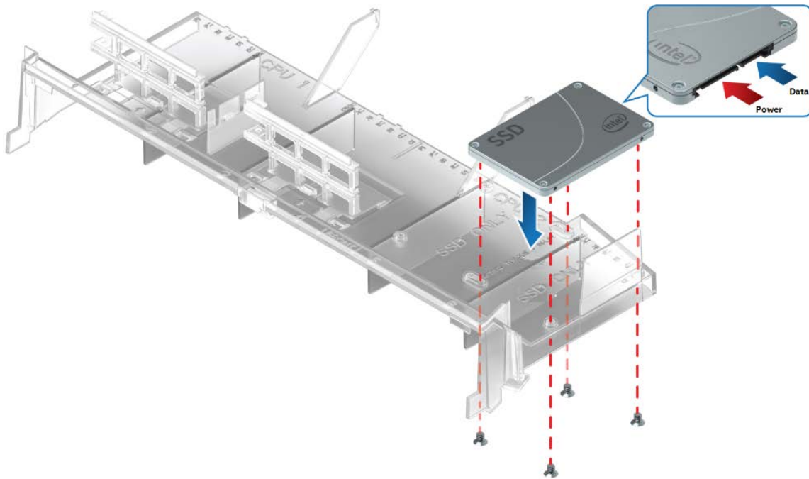
Figure 61. 2.5" Solid state drive (SSD) mounting option
