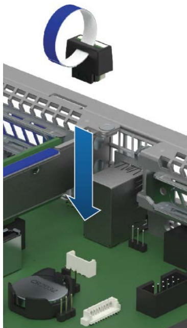
Figure 71. Intel® VROC upgrade key
