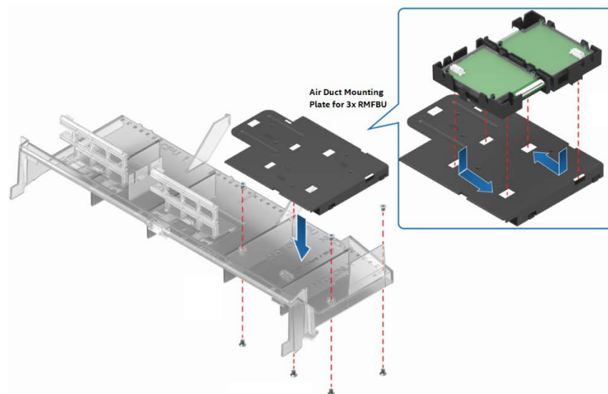
Figure 78. Triple RMFBU (default) mounting bracket installation
