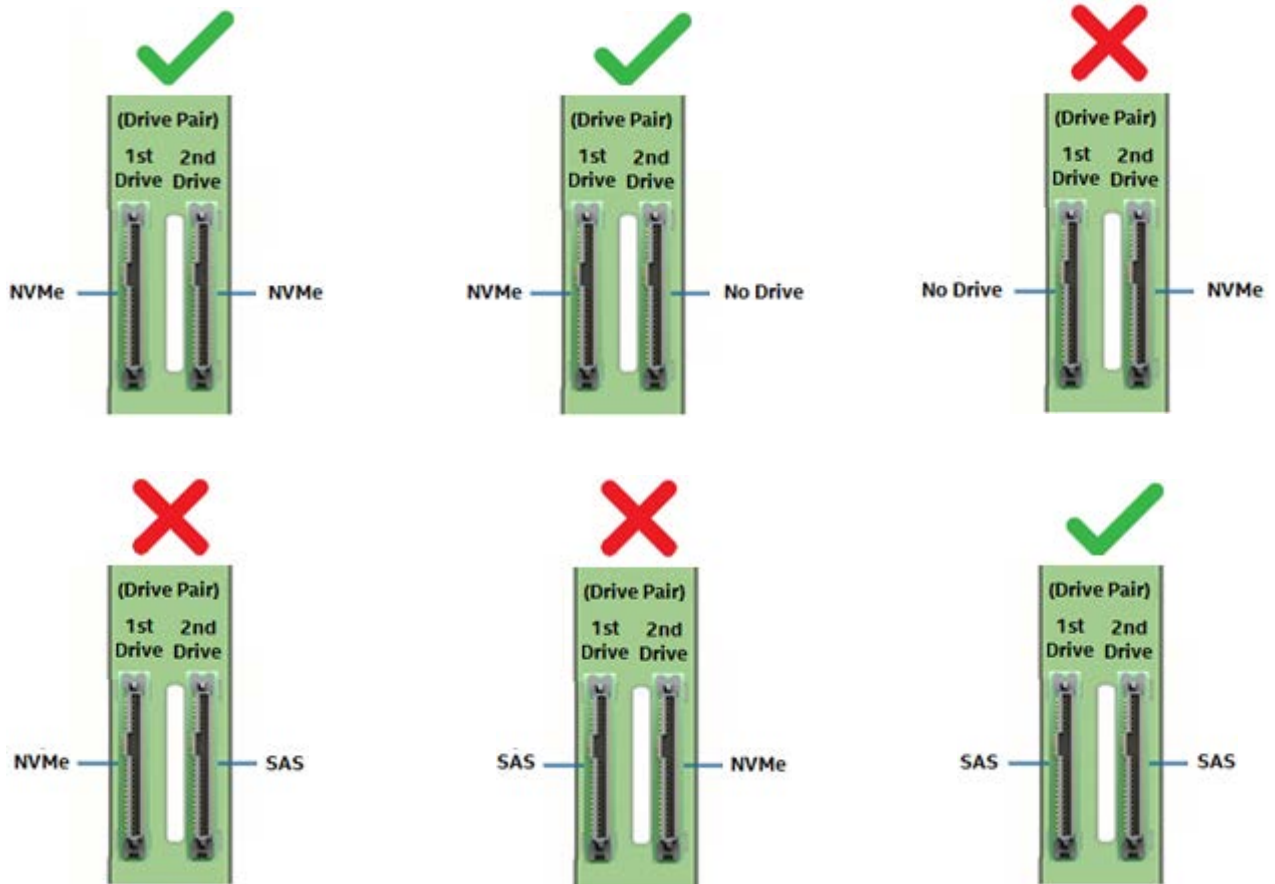
Figure 74. Supported drive population for onboard OCUlink connectors or tri-mode Intel® RAID module
