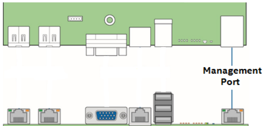
Figure 94. Dedicated management port
