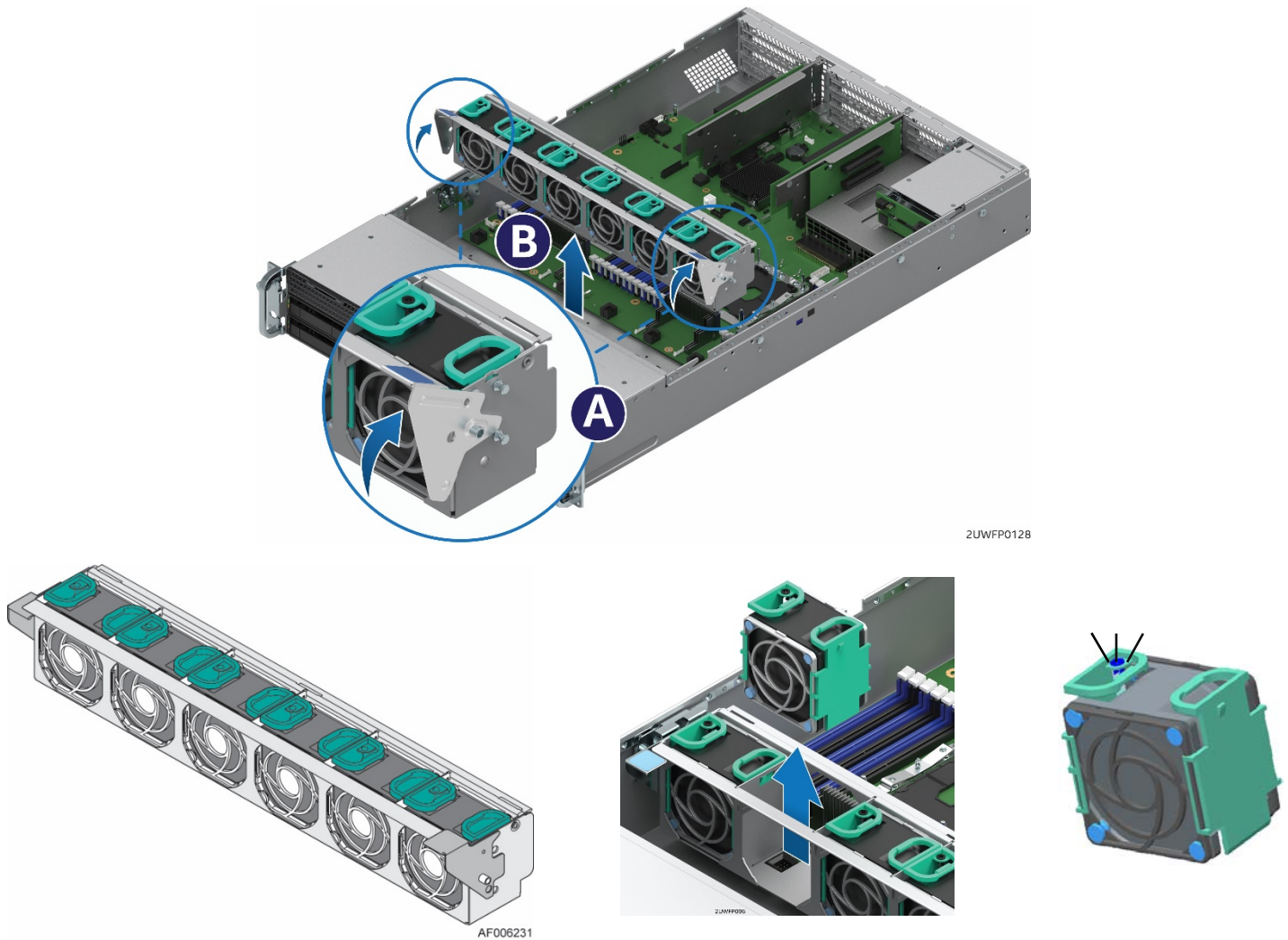
Figure 33. System fan assembly
