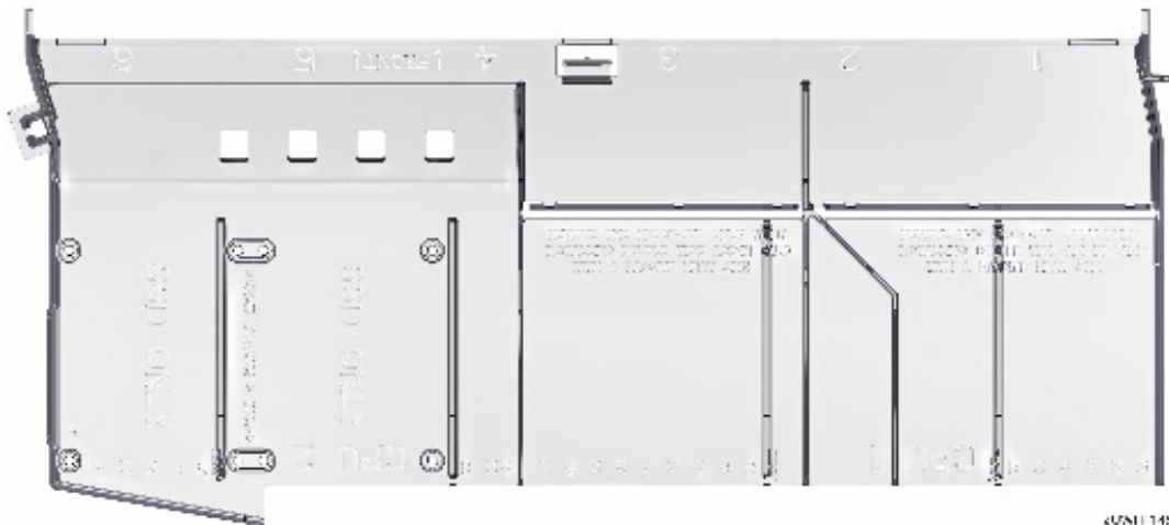
Figure 37. High airflow air duct included in accessory kit (iPC – AWFCOPRODUCTAD)
