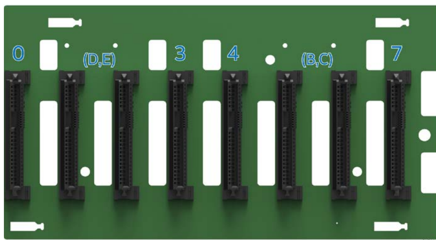
Figure 54. 8 x 2.5" dual-port SAS backplane, front side
