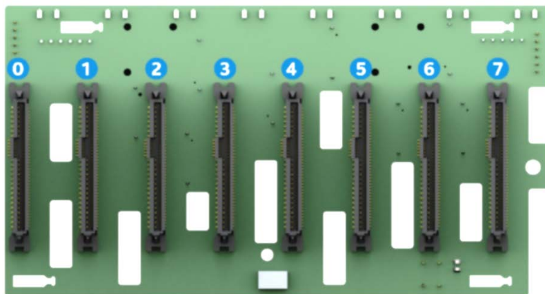
Figure 51. 8 x 2.5" SAS/SATA/NVMe* hot swap backplane, front side
