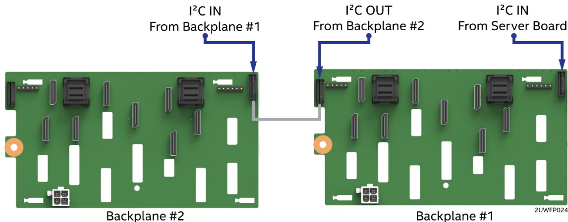
Figure 53. 8 x 2.5" dual port SAS backplane, back side
