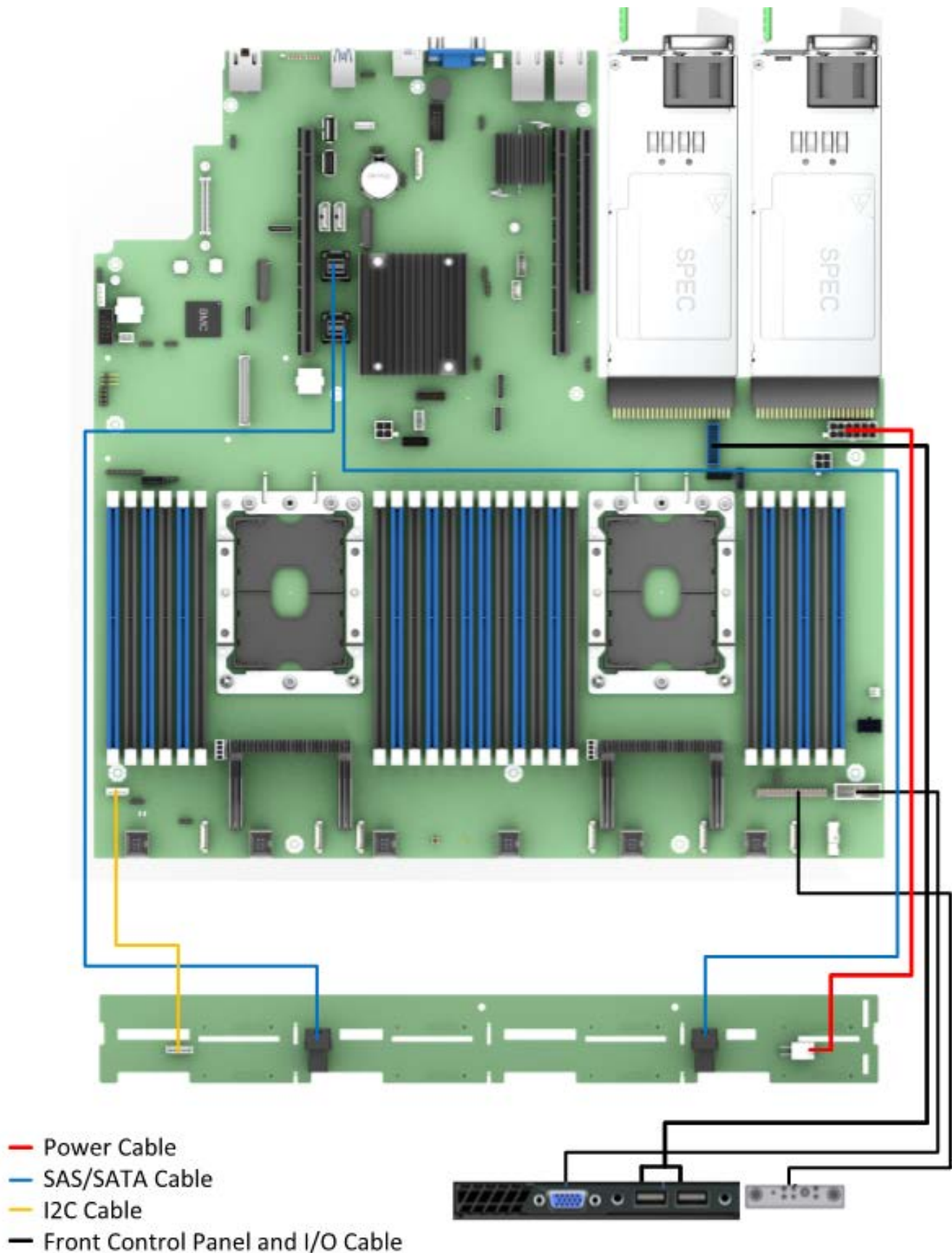
Figure 96. R2308WFxxx system cable routing diagram
